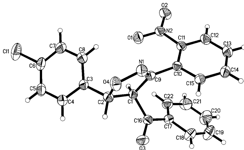
Figure 1. ORTEP diagram of compound 3a (probabilities of 30%), showing the atomic numbering scheme.
