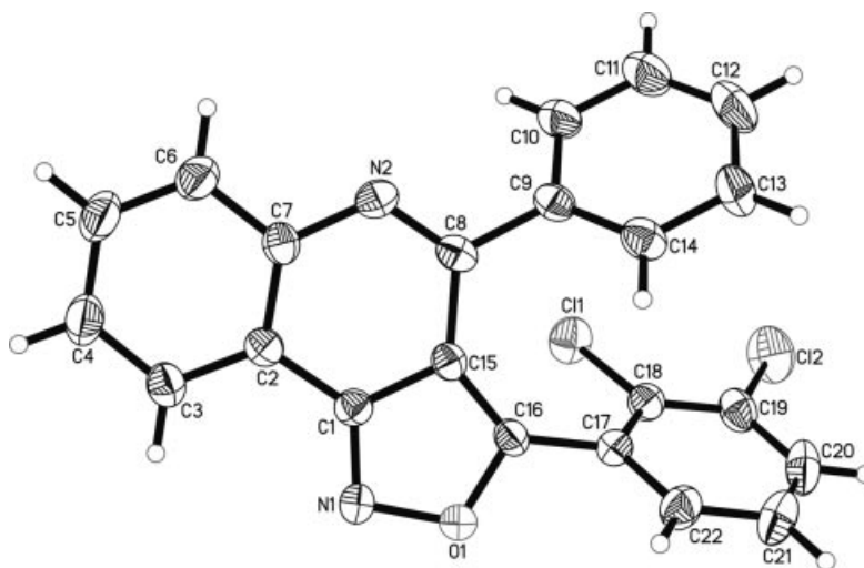
Figure 2. ORTEP diagram of compound 5c (probability of 30%), showing the atomic numbering scheme.
