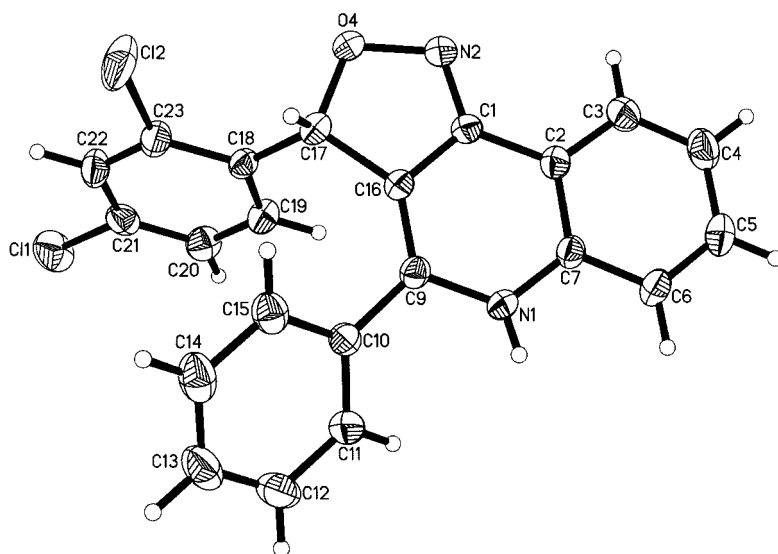
Figure 3. ORTEP diagram of compound 7d (probability of 30%), showing the atomic numbering scheme. A solvent molecule [(\text{CH}_3)_3\text{Si}-\text{Si}(\text{CH}_3)_3] has been omitted for clarity.
