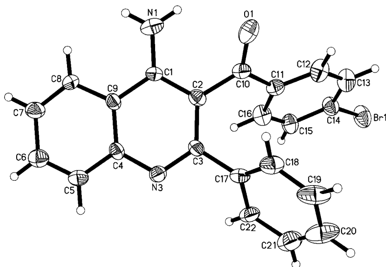
Figure 4. ORTEP diagram of compound 11b (probability of 30%), showing the atomic numbering scheme.
