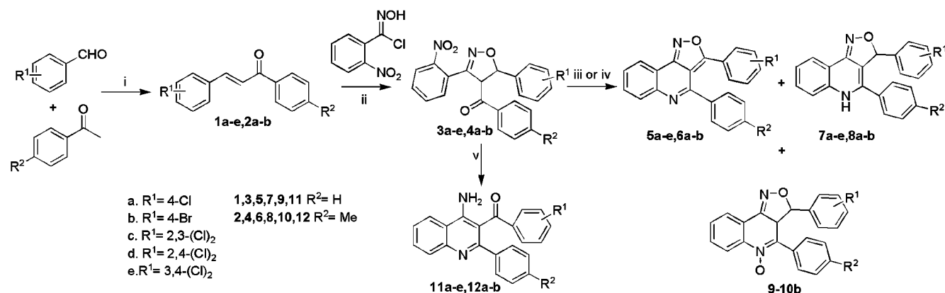
Scheme 1. Reagents and conditions: (i) aq. KOH, MeOH, 15–30 min. (ii) \text{Et}_3\text{N} , diethyl ether, -78^\circ\text{C} to room temp., 14–16 h. (iii) \text{SnCl}_2 \cdot 2\text{H}_2\text{O} , MeOH, reflux, 80^\circ\text{C} , 30 min. (iv) Pd/C (10%), 2.76 bar of \text{H}_2 , room temp., 30 min. (v) Fe, AcOH, reflux, 110^\circ\text{C} , 30 min.
